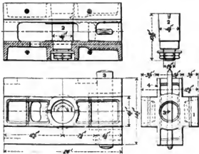
Figs. 1074-1077. Four-Guide Cross-head. Baldwin Locomotive Works.
